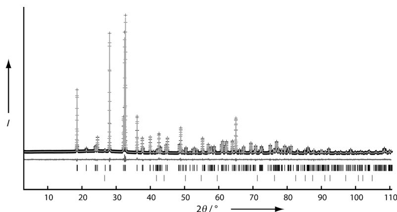
Figure 3. Observed (crosses) and calculated (light gray line) powder diffraction pattern of \gamma - \text{P}_4\text{N}_6(\text{NH}) as well as difference profile (dark gray line). Black vertical bars represent the positions of Bragg reflections of \gamma - \text{P}_4\text{N}_6(\text{NH}) and gray vertical bars the Bragg reflections of hexagonal BN.
